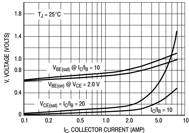
Figure 9. "On" Voltage
